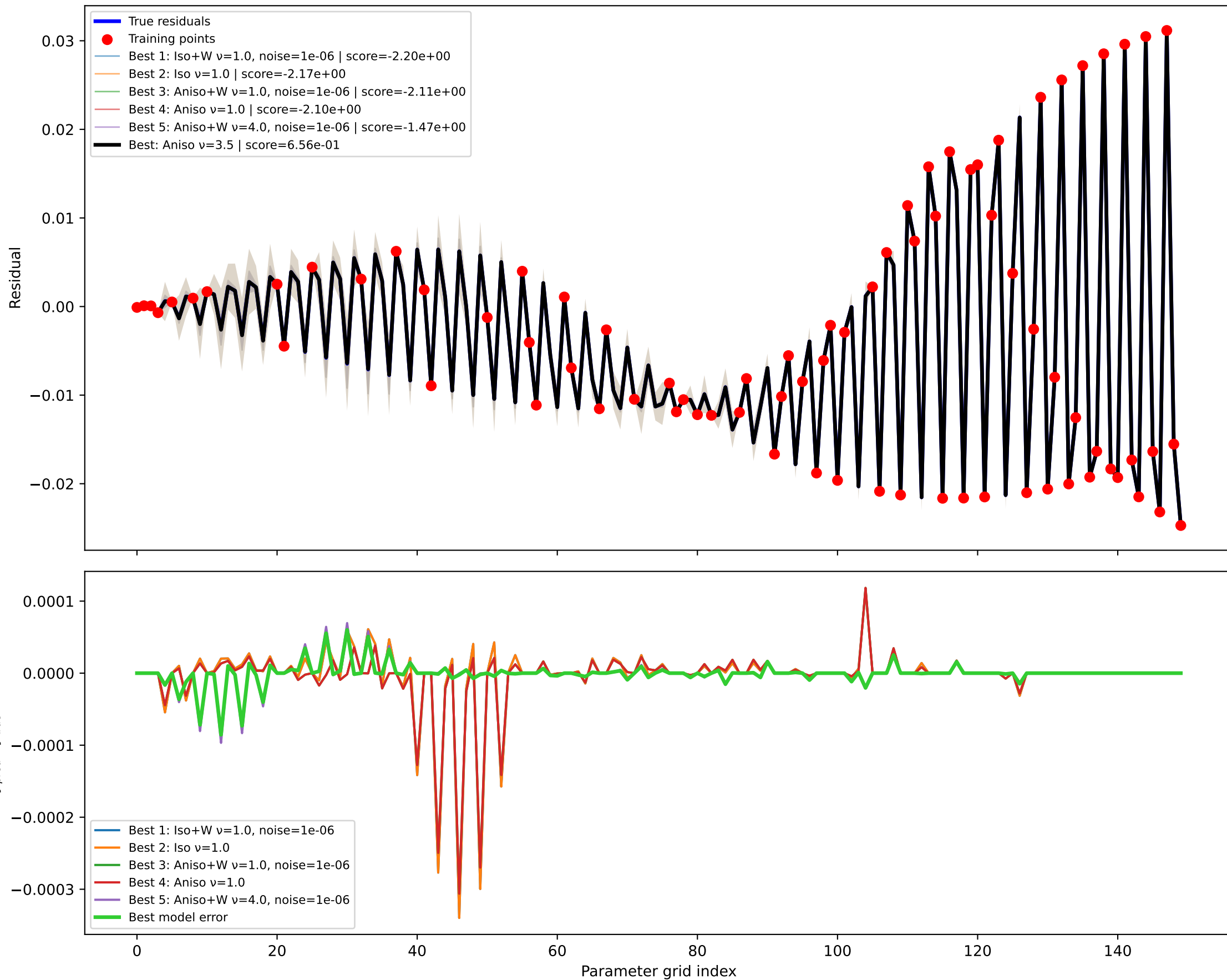
GPR kernel comparison node=9 RMSE=1.557e-05, train RMSE=2.076e-10
